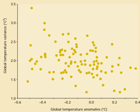
Figure 1: Inter-annual surface temperature variability vs. global temperature anomalies for the 1877–1997 time series showing the warmer the surface temperature, the less variable the climate becomes
